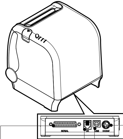
INTERFACE CONNECTOR
